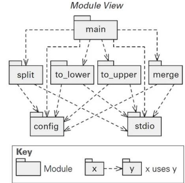
Module View
