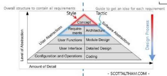
Style → Concept / Tactic → Architecture
