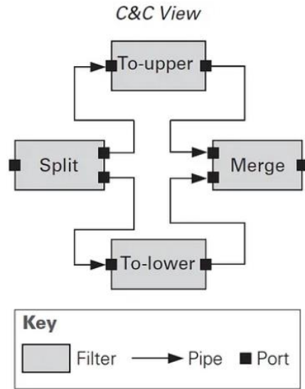
C&C View
