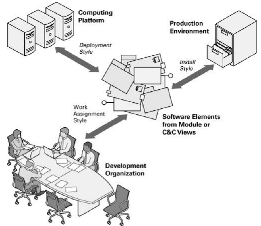
[3가지 Allocation Style] Deployment · Install · Work Assignment
